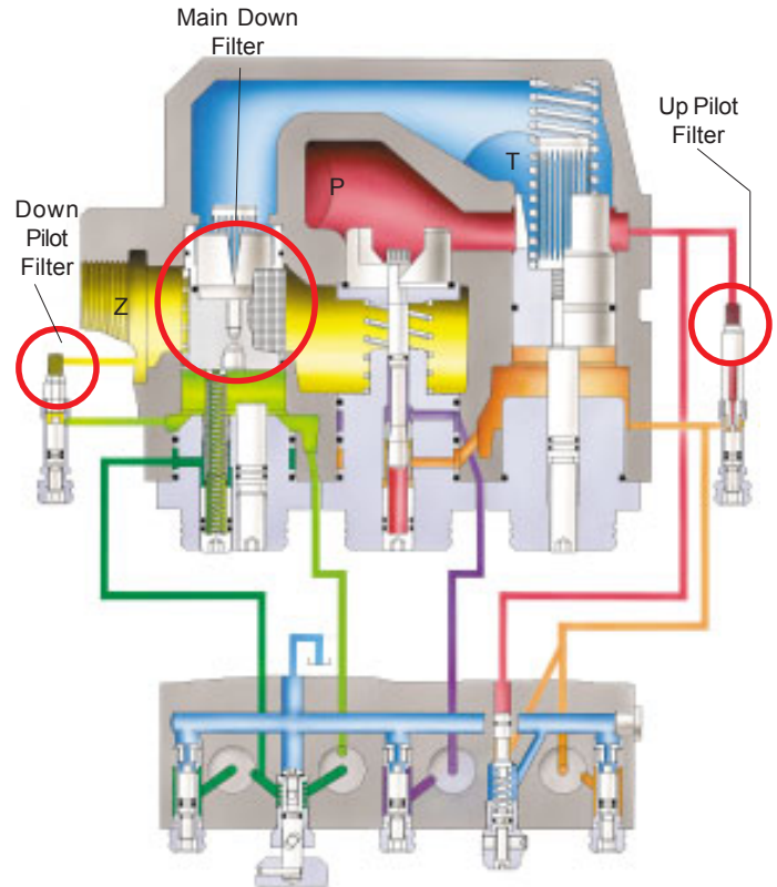
BLAIN EV 100 Elevator Valve
