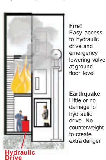
Hydraulic Elevator (Passenger freed)
